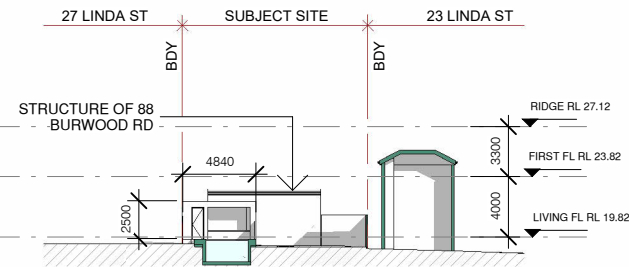
7 WEST ELEVATION 2 - POOL EQUIPMENT 1 : 500
