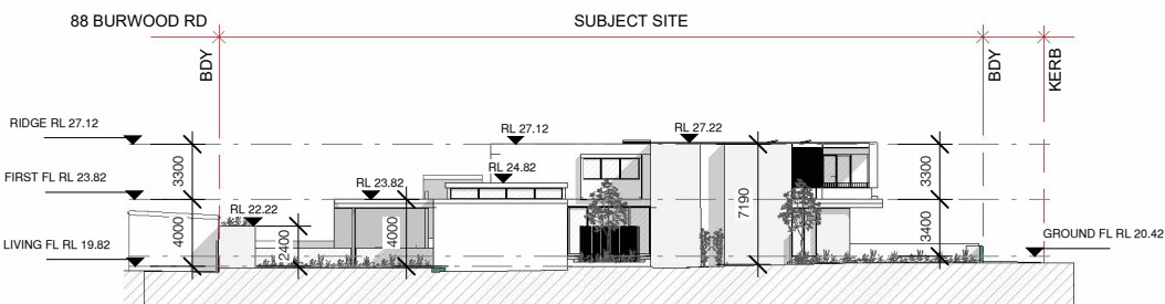
4 NORTH ELEVATION 1 : 500
