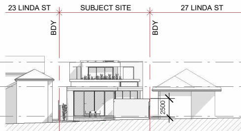
6 EAST ELEVATION 2 1 : 500
