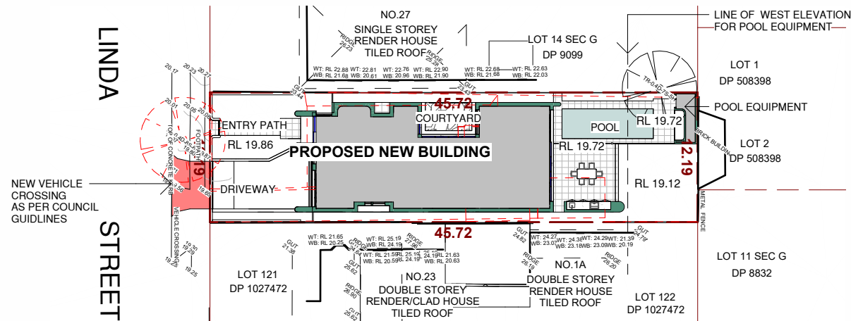
1 NOTIFICATION PLAN 1 : 500
