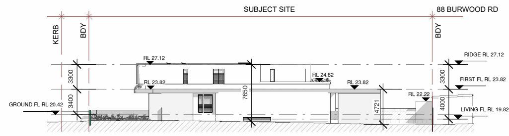
5 SOUTH ELEVATION 1 : 500
